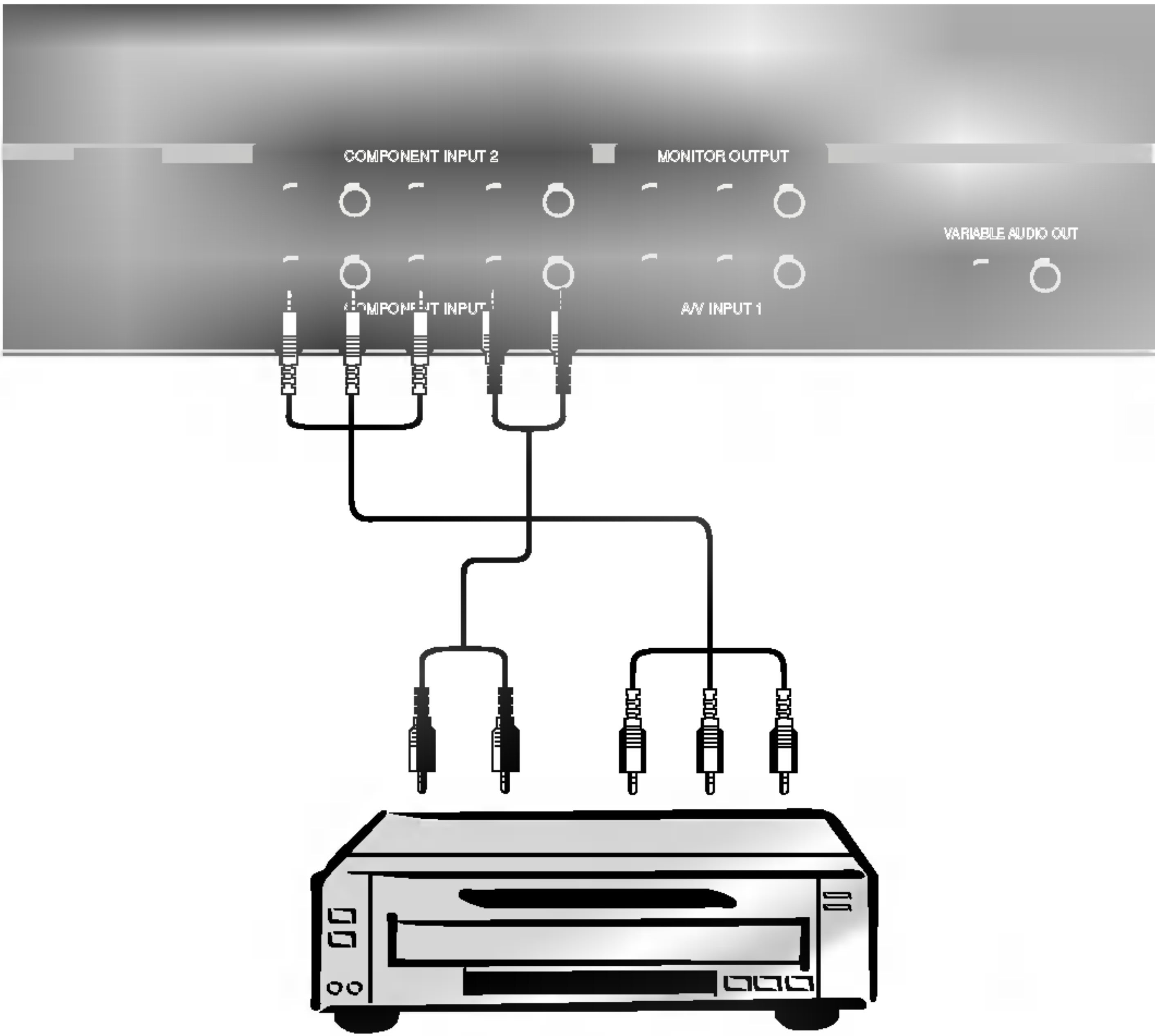
< Back panel of the set >
