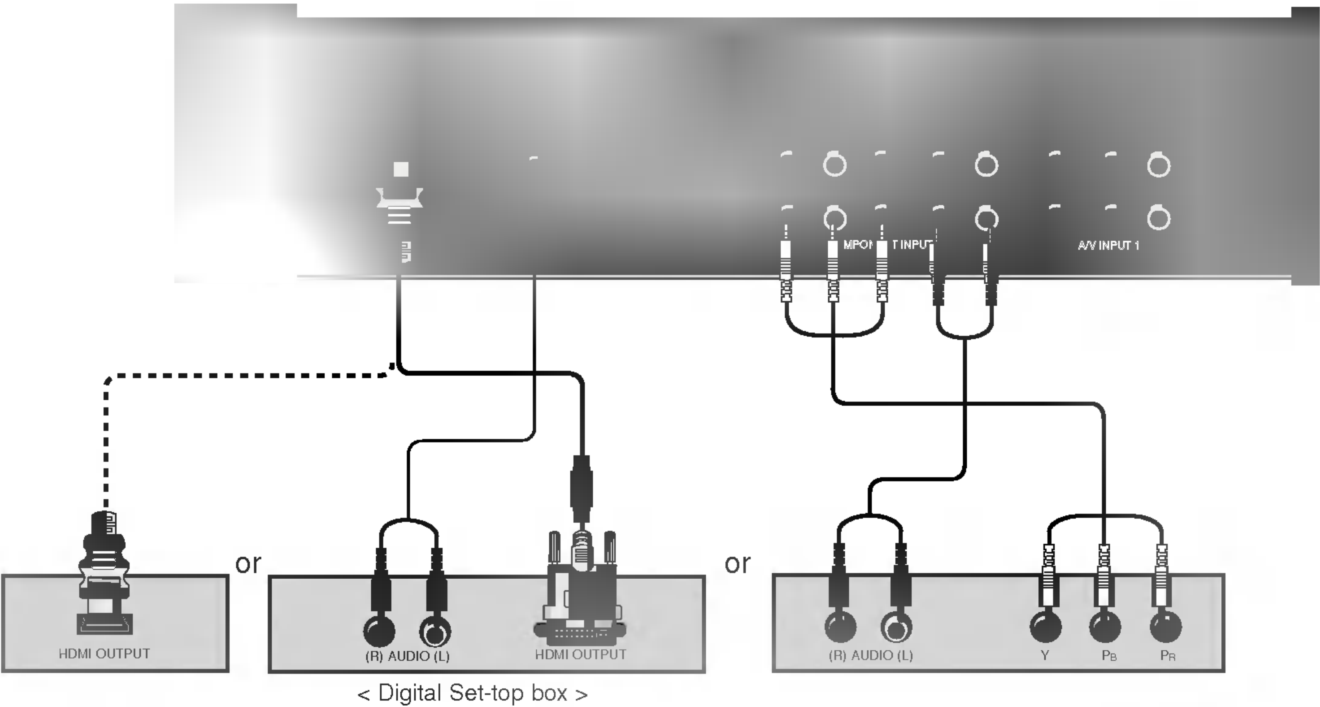
< Back panel of the set >
