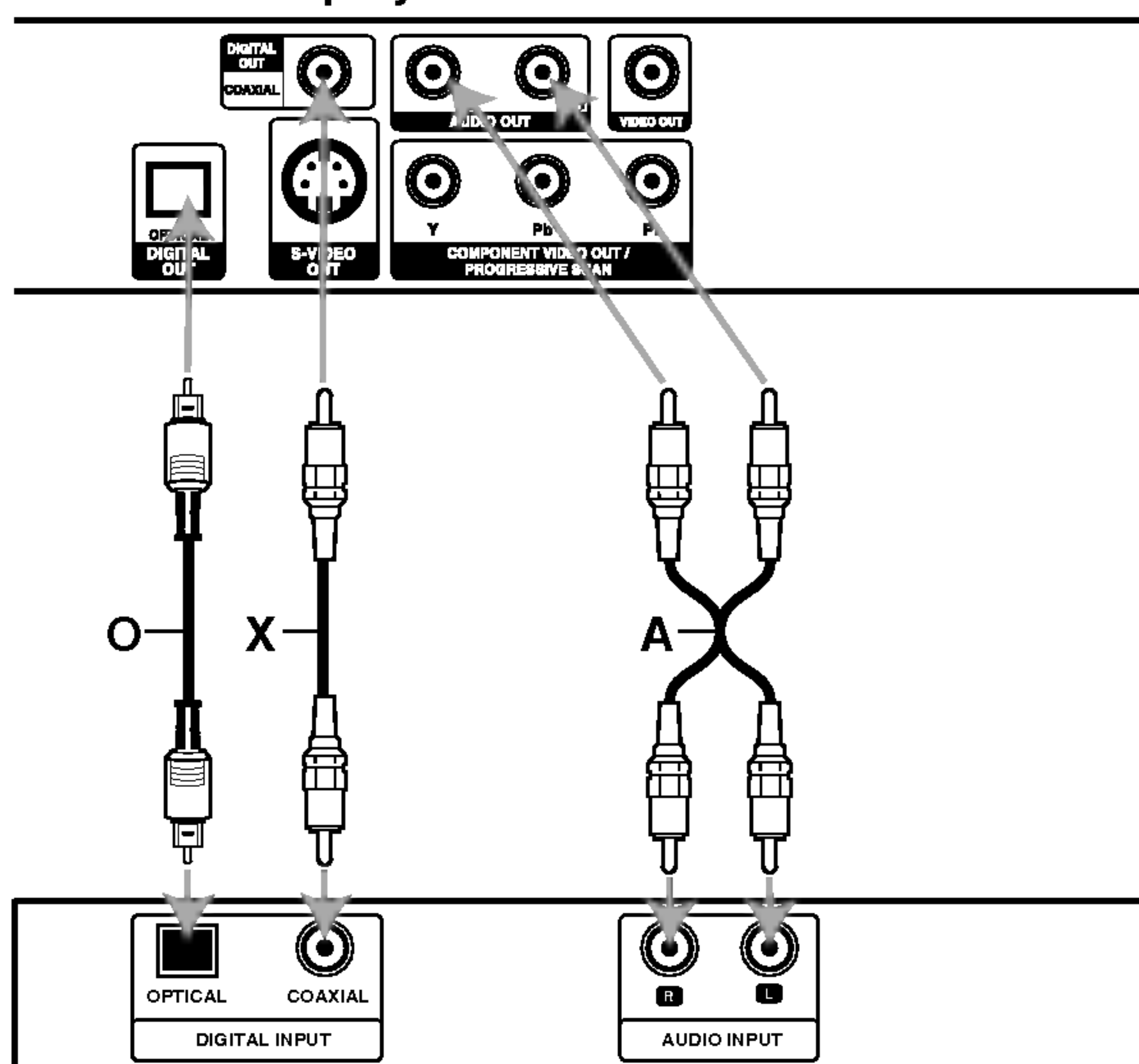
Amplifier (Receiver)
