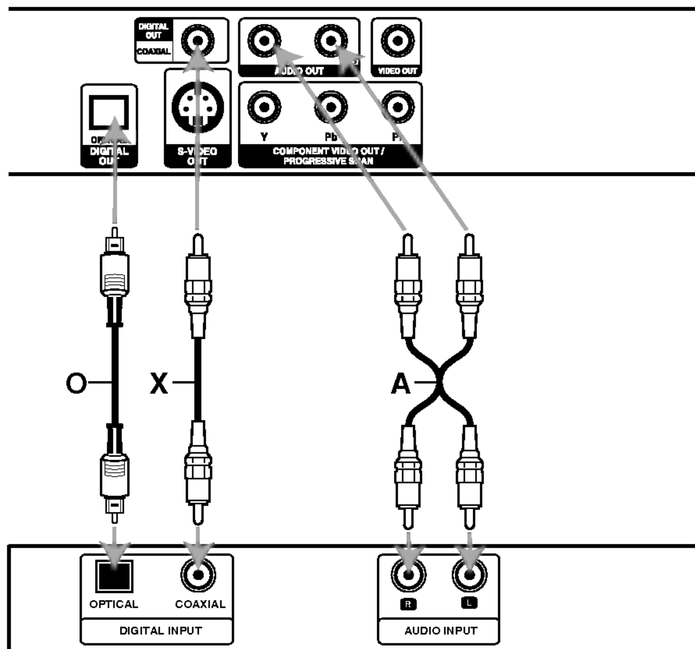
Pojačalo (Receiver)
