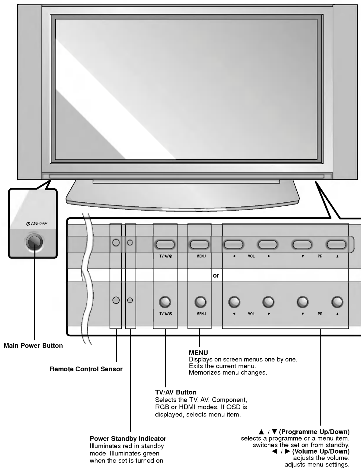
<Front Panel Controls>
