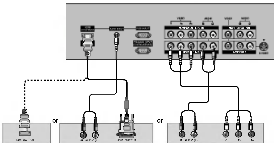
< Digital Set-top box >
