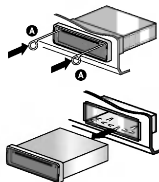
Panel frontal
