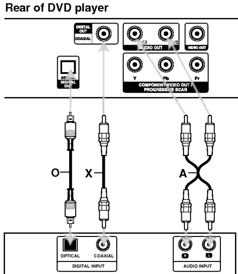
Amplifier (Receiver)
