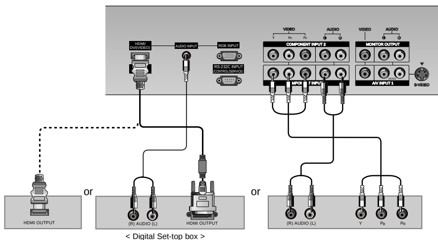
< Digital Set-top box >
