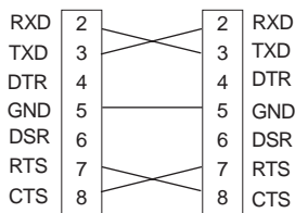
<Fig.1, RS-232 Interface Cable>
