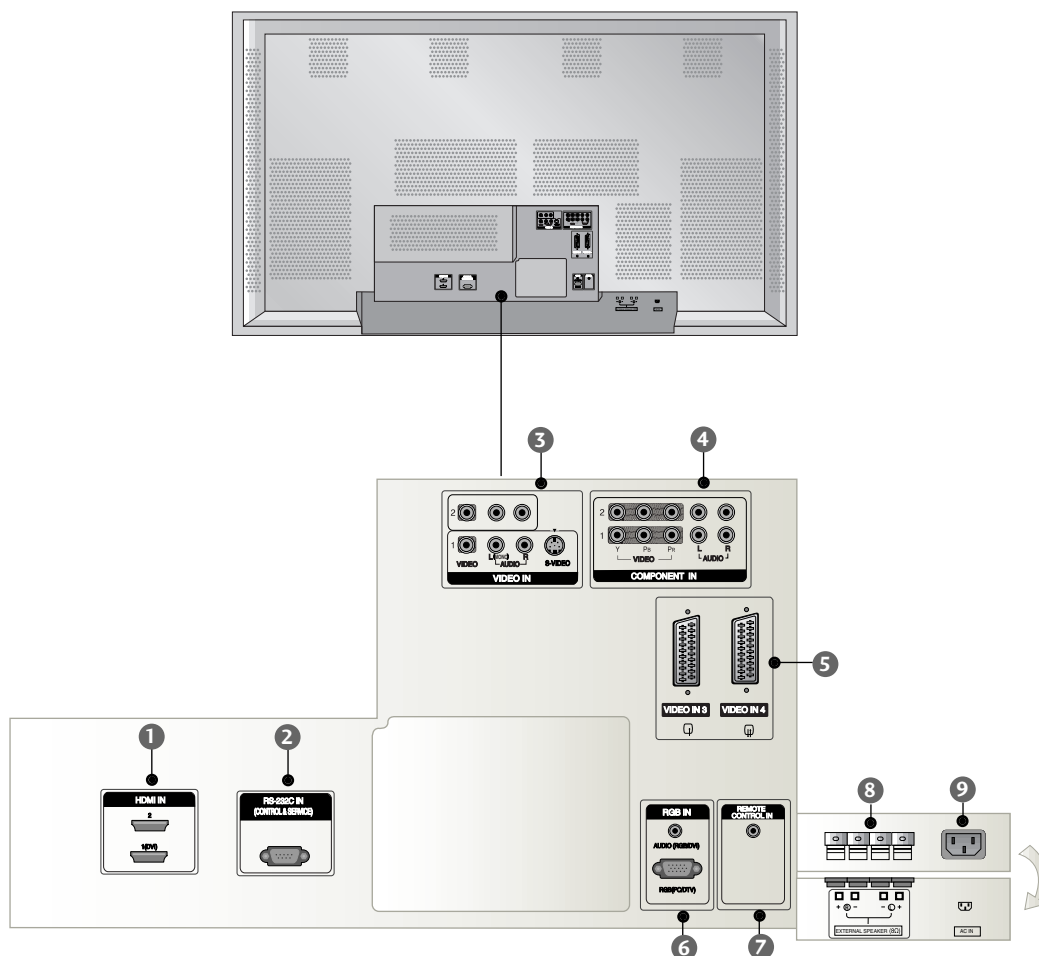
Back Connection Panel
