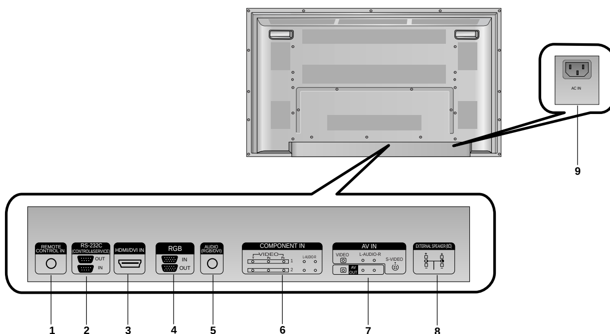
Back Connection Panel
