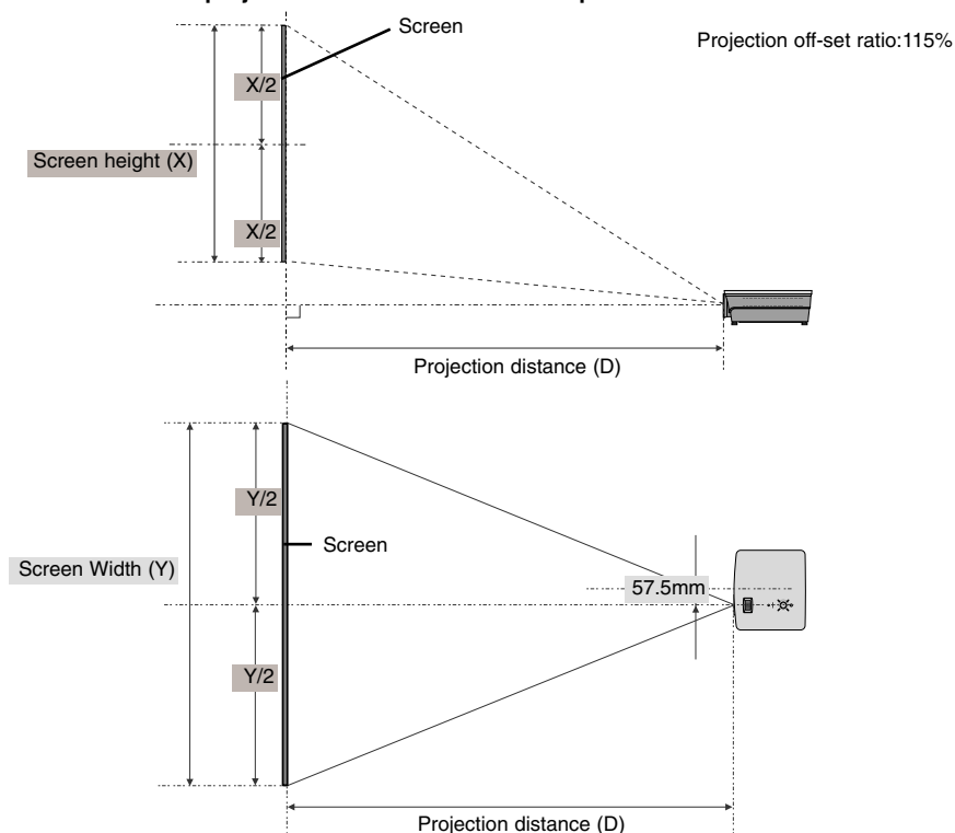
projection distance based on the picture format
