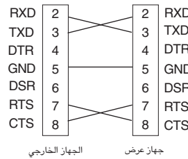
<Fig.1, RS-232 Interface Cable>
