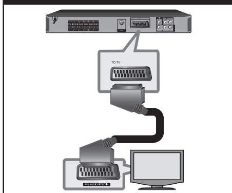
SCART Connection
