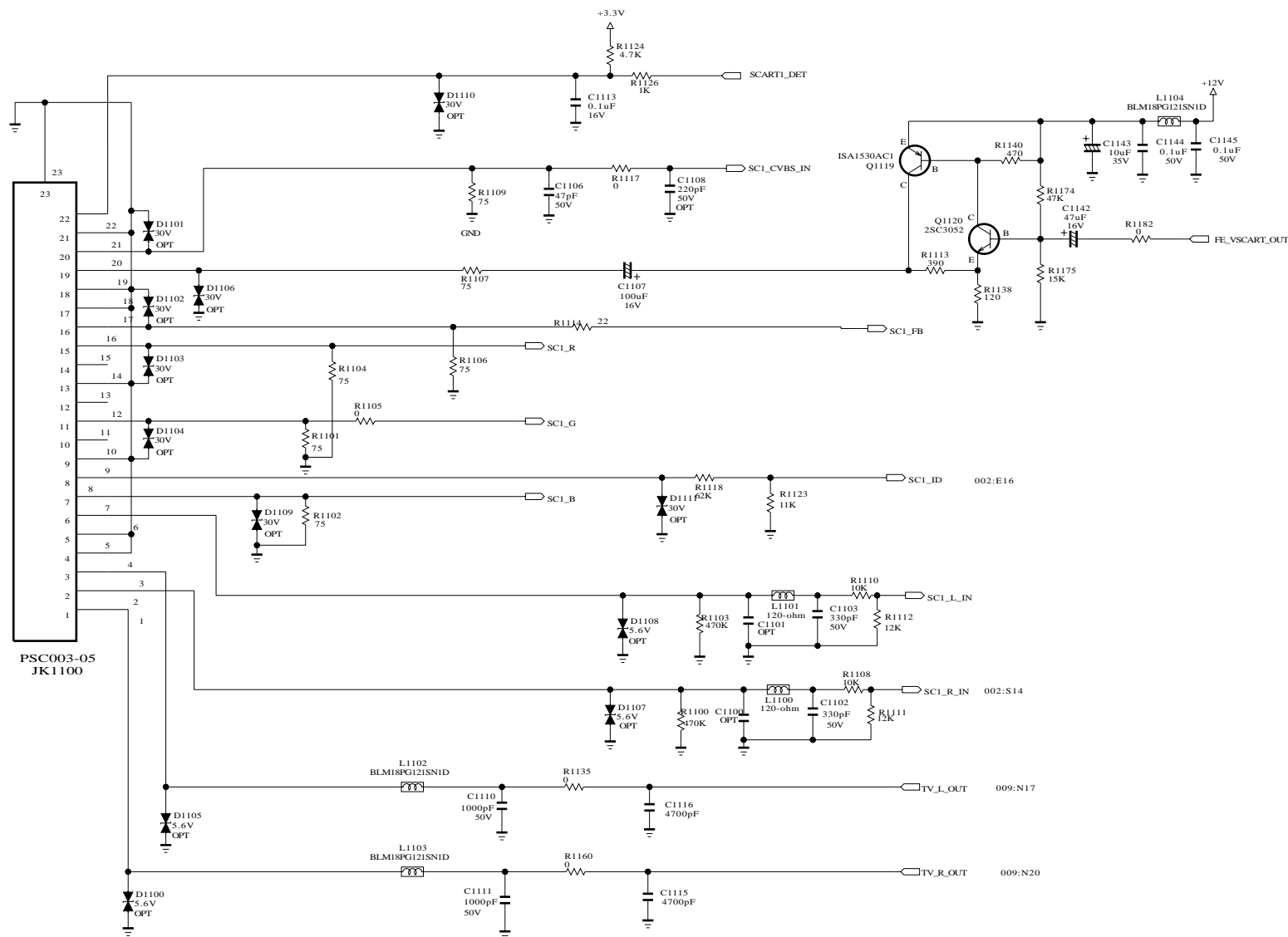
[SCART2 PIN 8]
