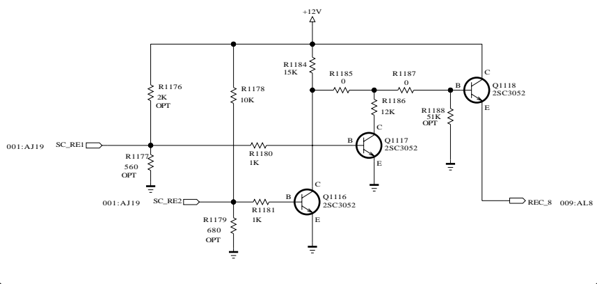
[SCART2 PIN 8]
