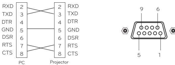
<Figure 1, RS-232 connection diagram>
