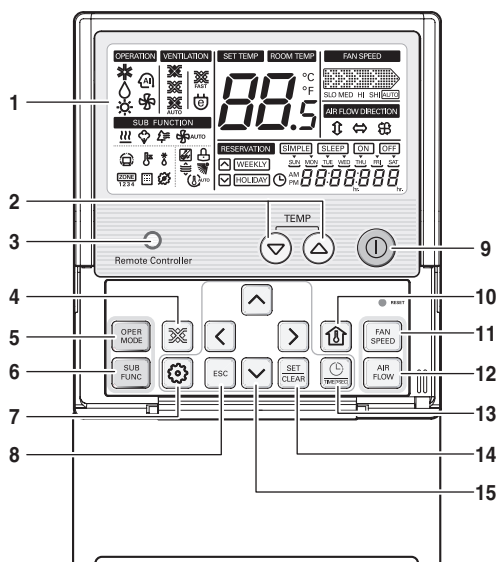
Wired remote controller: PQRCSA1
