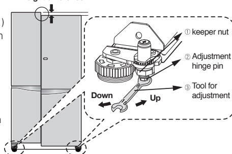
Height difference
