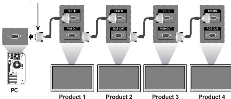
15-pin D-Sub Signal Cable
