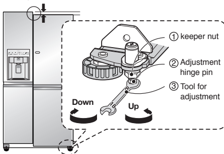
Height difference
