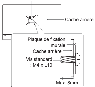
Plaque de fixation murale
