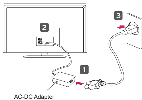
AC-DC Adapter
