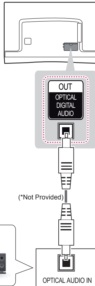
Digital Audio System / Canvas Speaker (Only EA88**)
