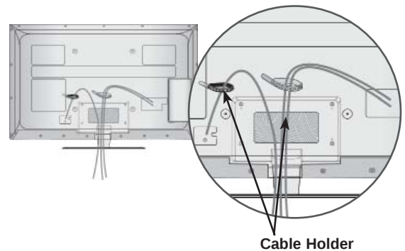
Cable Holder
