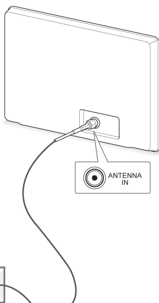
Wall Antenna Socket
