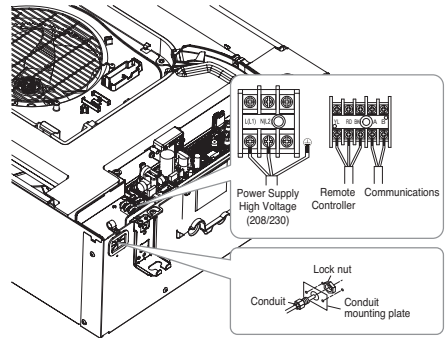
TS Chassis
