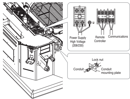
TM-A/TP-B Chassis
