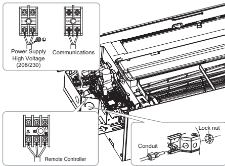
TC Chassis
