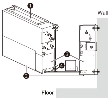
Case 2. Installation on the wall
