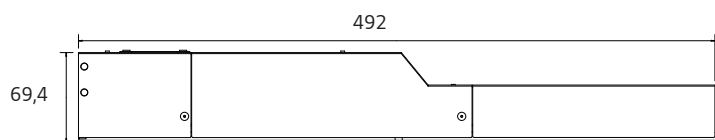
ACC-14LATB3, ACC-LTA14V1, ACC-LTA14W1, ACC-LTA14U1
