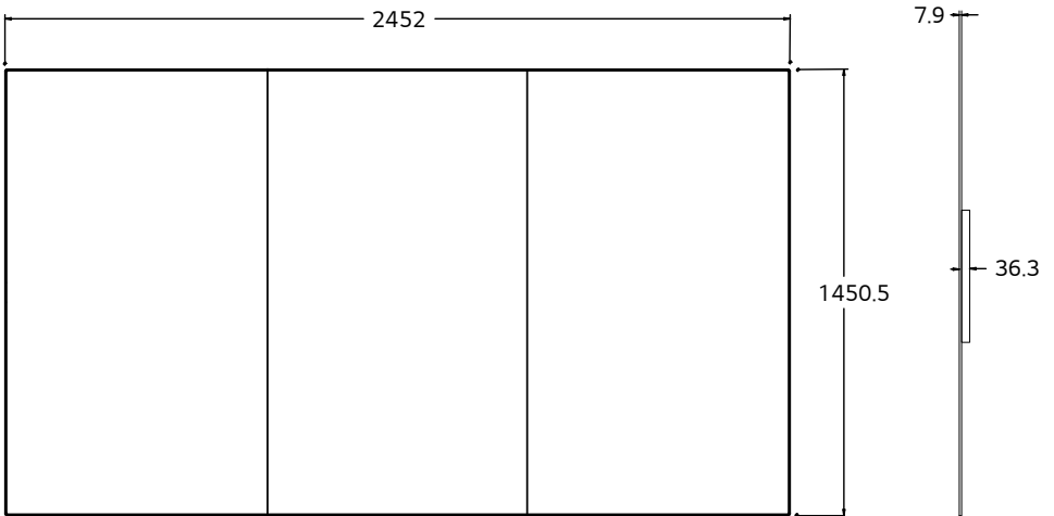
65EV5C-3 (1 x 3)
