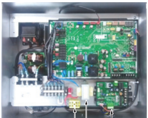
VWFC PCB Transformer Terminal block
