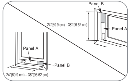
For window openings from 24"(60.9 cm) to 38"(96.52 cm), use the window vent panel (Panel A) and an extension panel (Panel B).
