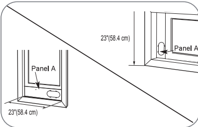
For an 23"(58.4 cm) window opening, use the window vent panel (Panel A) by itself.
