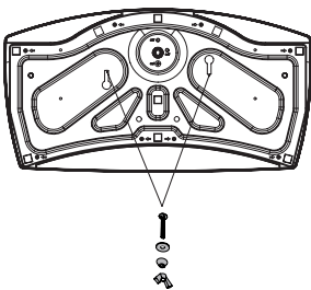
2-Screws, 2-Washers, 2-Nuts (provided as parts of the product.)
