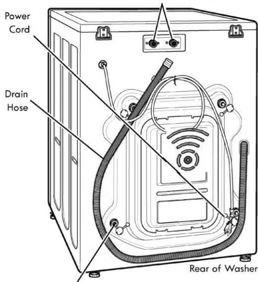
Cold and Hot Water Inlets
