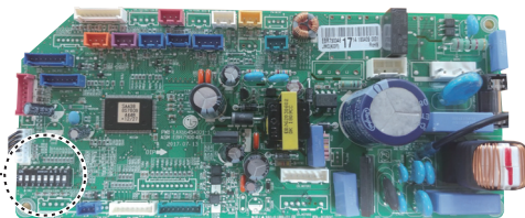
Interior PCB
