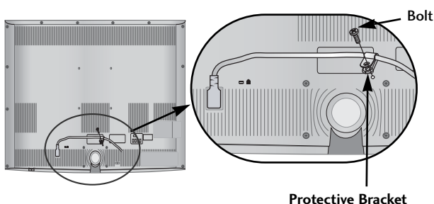
Protective Bracket
