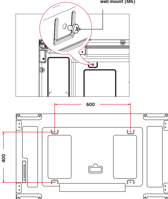
Screws for attaching the VESA wall mount (M6)
