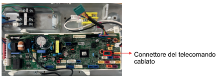
Remote Controller Connector (CN_REMO)
