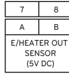
Terminal Block 1 (In Backup Heater)
