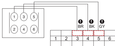
Terminal block 3 (Indoor Unit)
