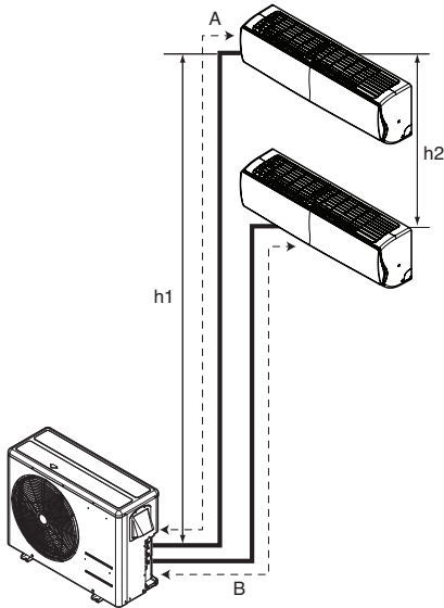
Type multituyaux
